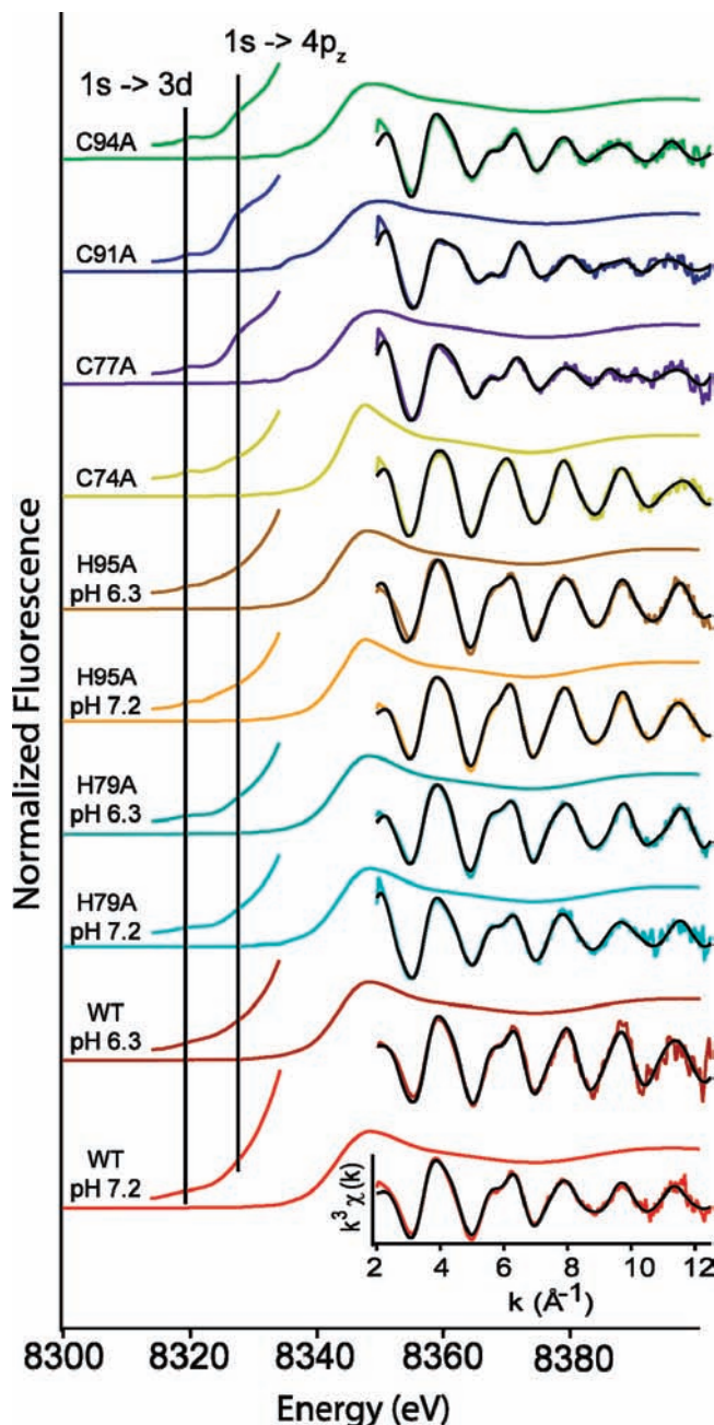
Figure 7. Nickel K -edge XAS data for holo-HypA proteins. XANES is shown as a single colored line. Left side is an expansion of the pre-edge XANES region. Right side is the unfiltered k^3 -weighted EXAFS data (colored line) and fits from Table 3 (black line).
