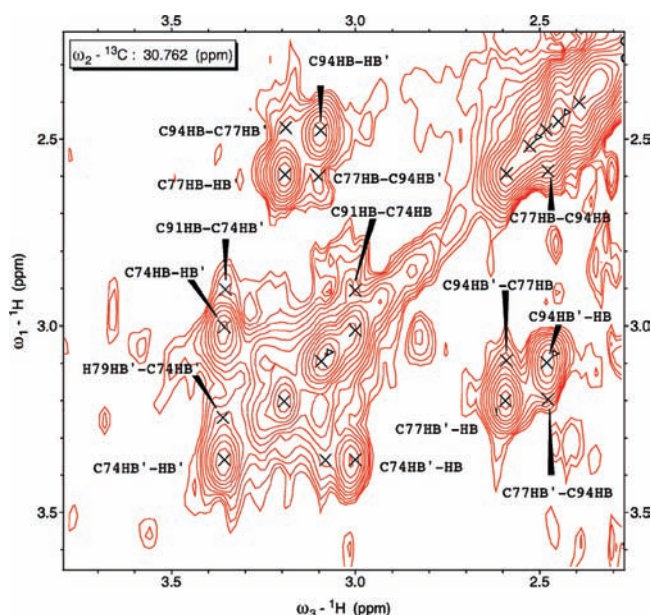
Figure 3. A plane from ^{13}\text{C} -edited three-dimensional ^1\text{H},^1\text{H} NOESY (800.13 MHz ^1\text{H} ) showing \beta - \text{CH}_2 NOEs between Zn-ligating Cys residues in HypA as described in the text.
