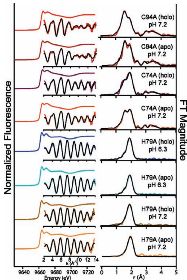
Figure 6. Zinc K -edge XAS data for selected mutant HypA proteins. Left: Normalized XANES spectra with unfiltered k^3 -weighted EXAFS spectra (colored line) and best fits (black line) from Table 2. Right: Fourier-transformed EXAFS spectra and fits. Data for other Cys \rightarrow Ala, Cys \rightarrow Asp, and H95A are shown in the Supporting Information.
