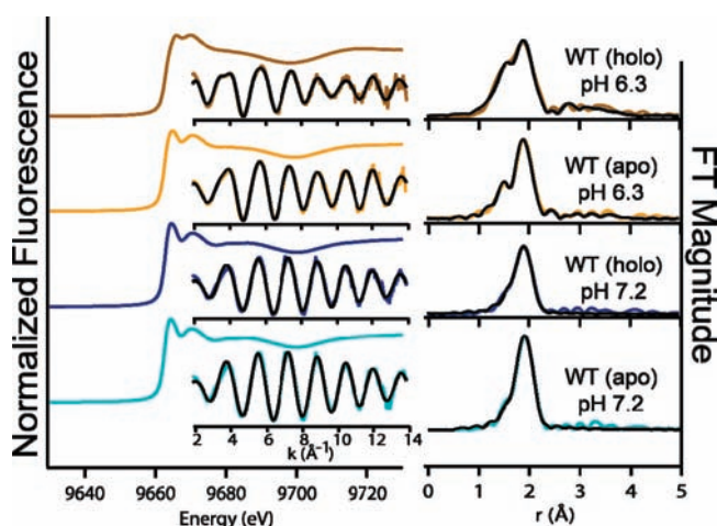
Figure 5. Comparisons of Zinc K -edge XAS of apo- and holo-WT-HypA at pH 7.2 and pH = 6.3. Left: Normalized XANES data with unfiltered k^2 -weighted EXAFS spectra (colored line) and best fits (black line) from Table 2. Right: Fourier-transformed EXAFS spectra and fits.
